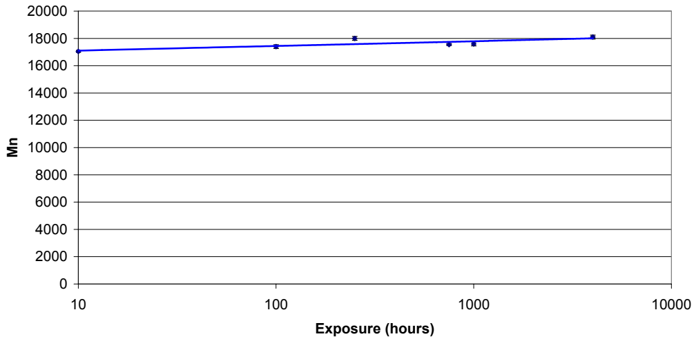
Number Average Molecular Weight: Centriforce Black
