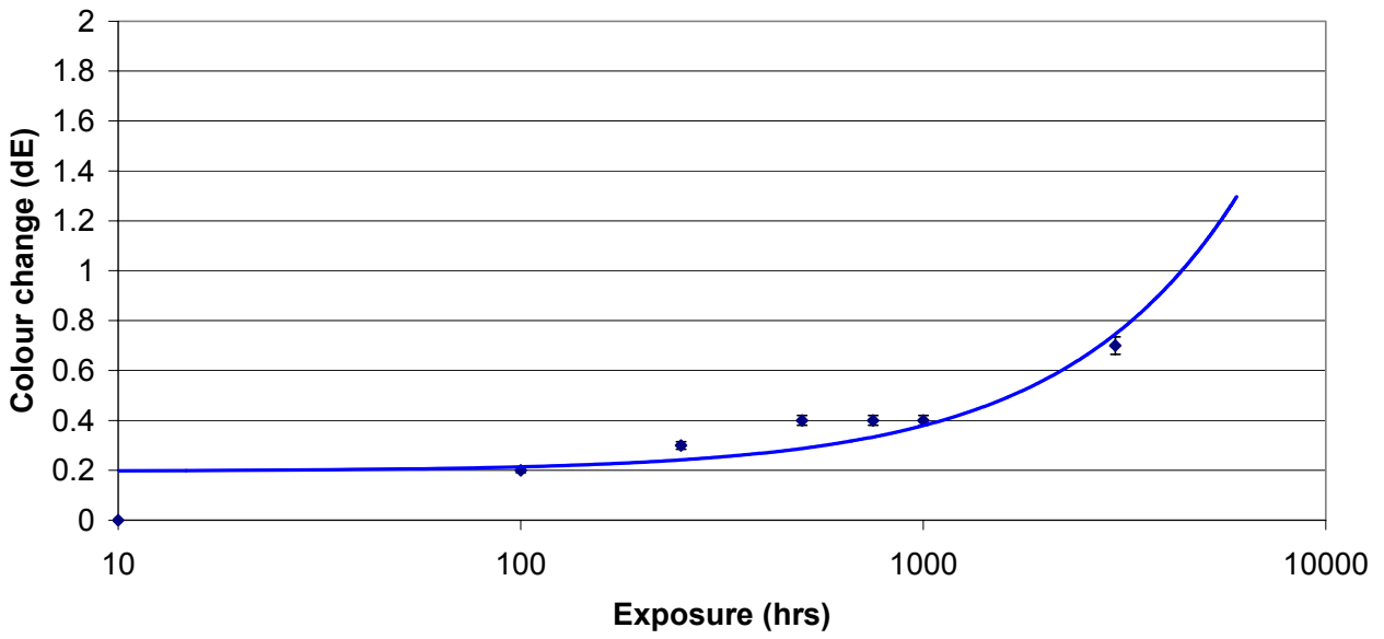
Colour change: Centriforce Black
