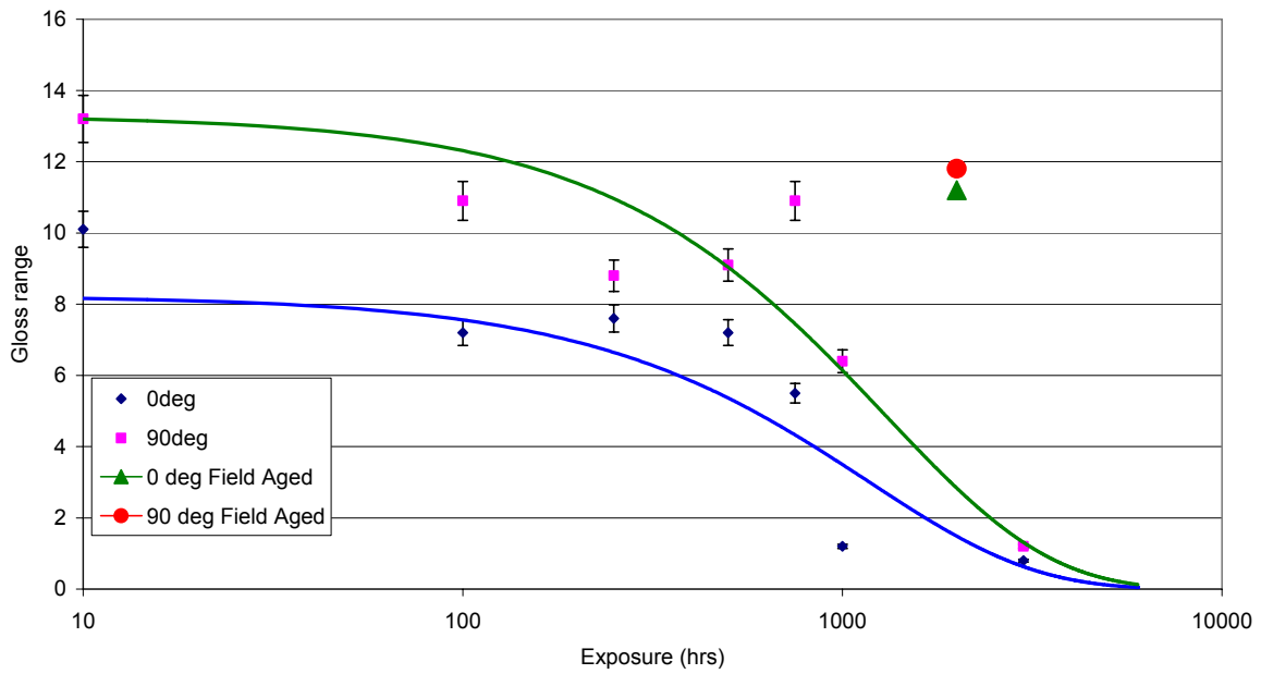
Gloss measurement: BPI Square
