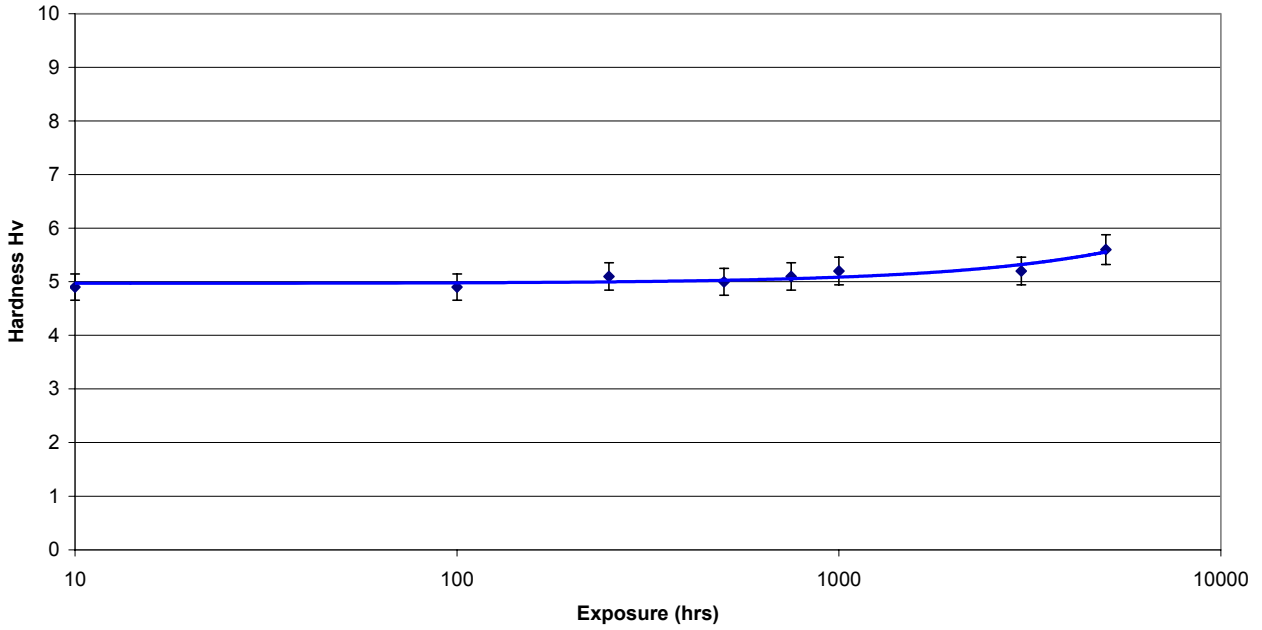
Vickers micro-hardness : Wheelie Bin Green
