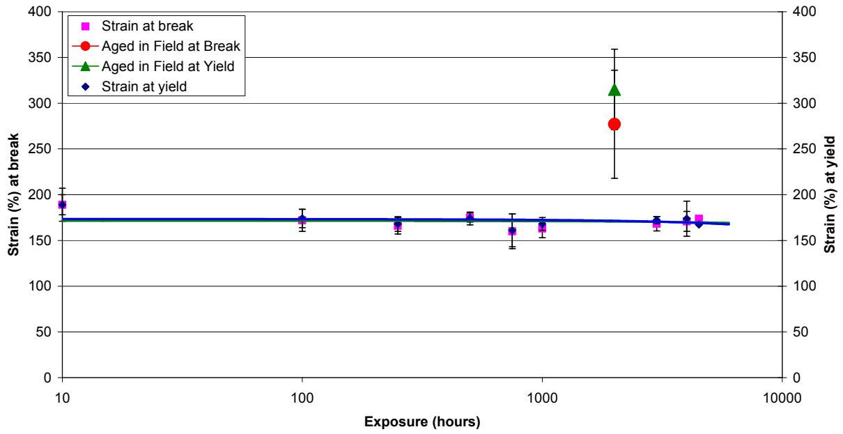
Tensile Strain: BPI Rectangular
