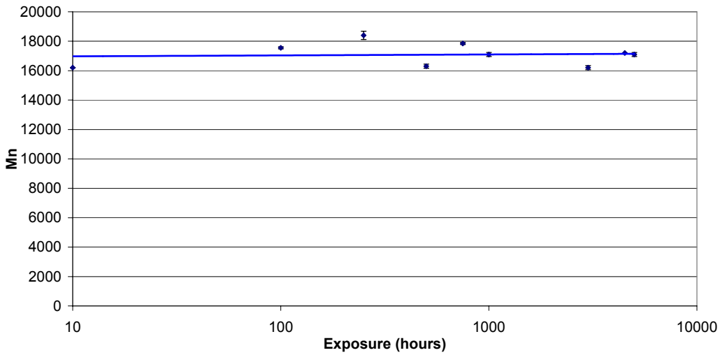
Number Average Molecular Weight: Centriforce Blue
