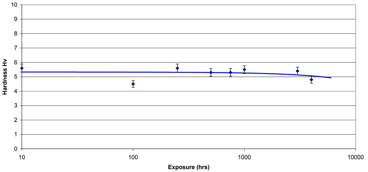
Vickers micro-hardness : Centriforce Black
