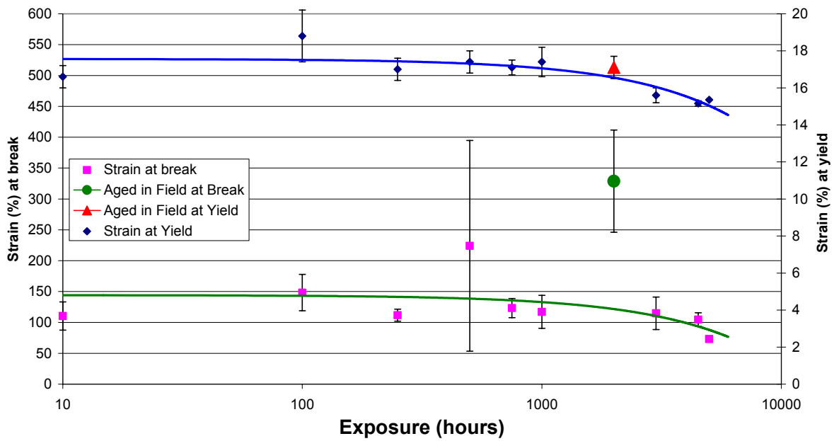
Tensile Strain: Centriforce Brown
