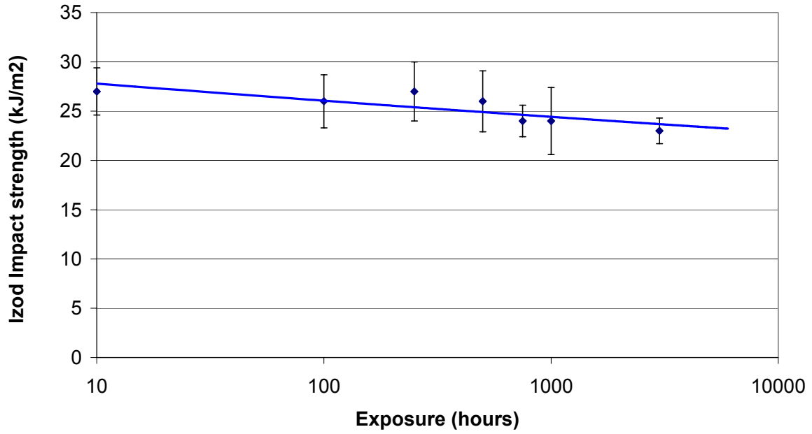
Izod Impact Strength: Centriforce Black
