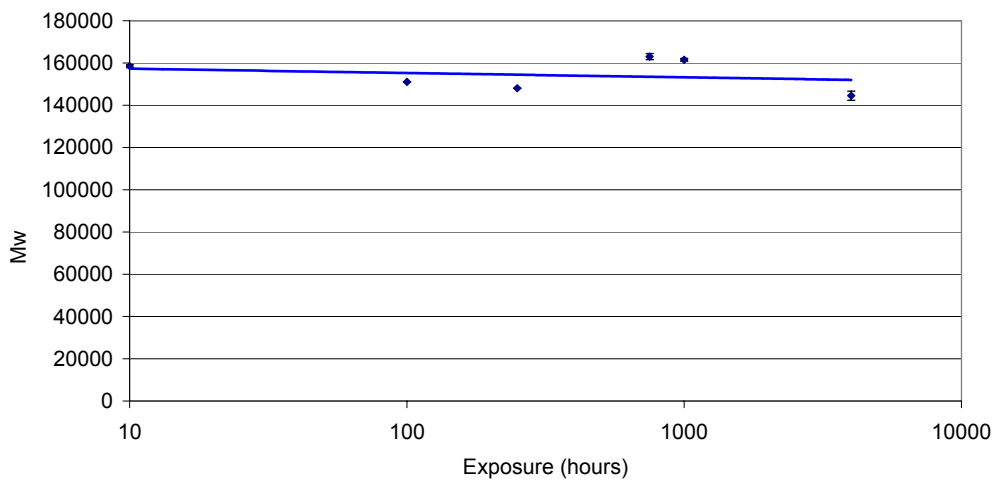
Weight Average Molecular weight: Centriforce Black
