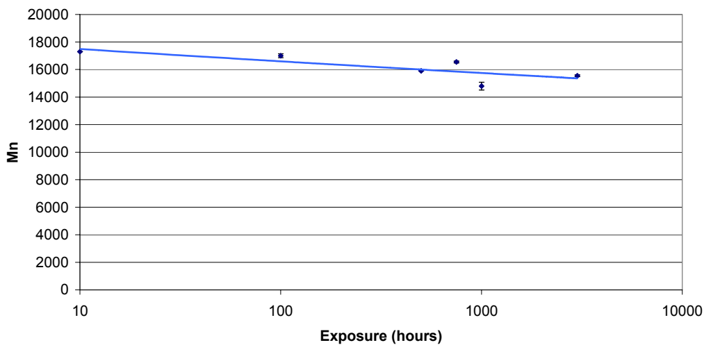
Number Average Molecular Weight: Wheelie Bin Black
