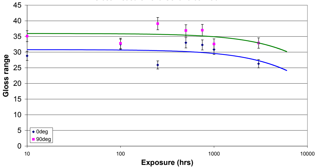
Gloss measurement: Centriforce Black
