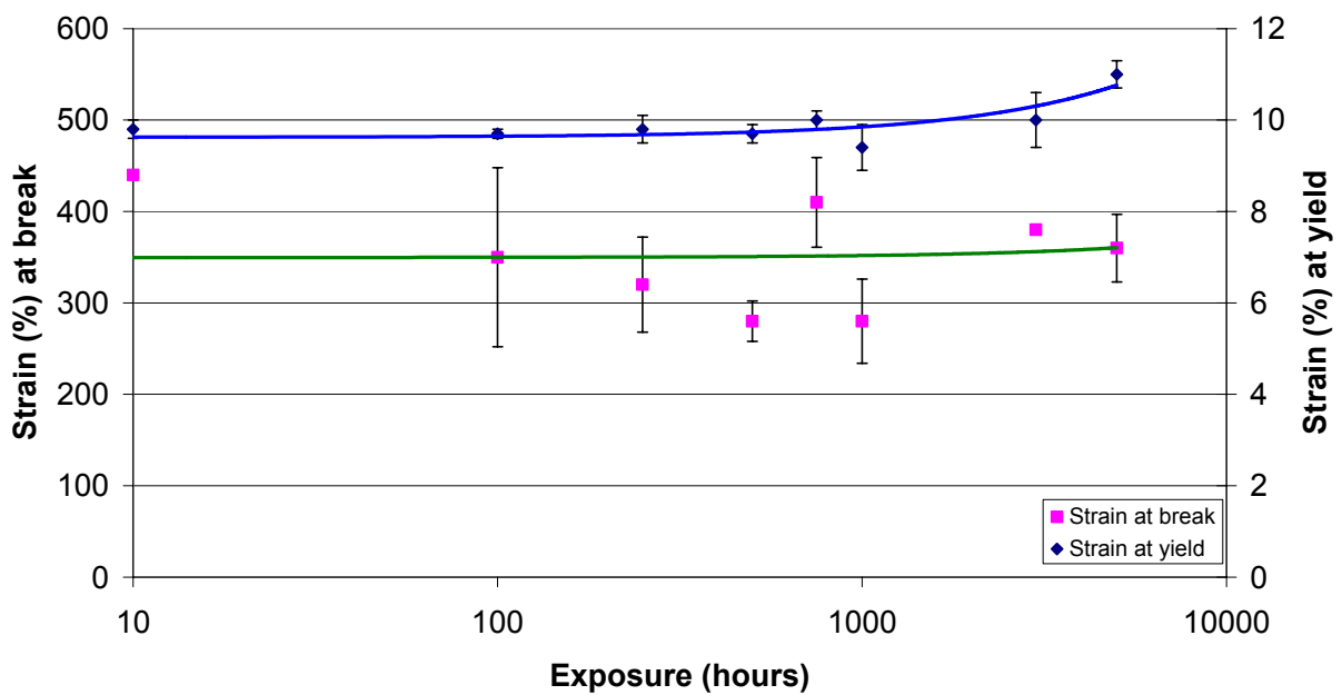
Tensile Strain: Wheelie Bin Green
