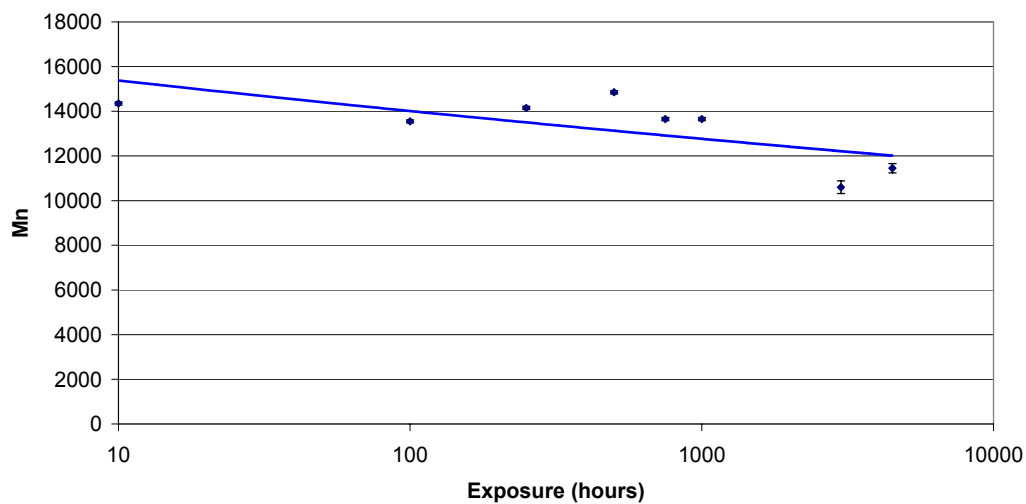
Number Average Molecular Weight: Centriforce Brown
