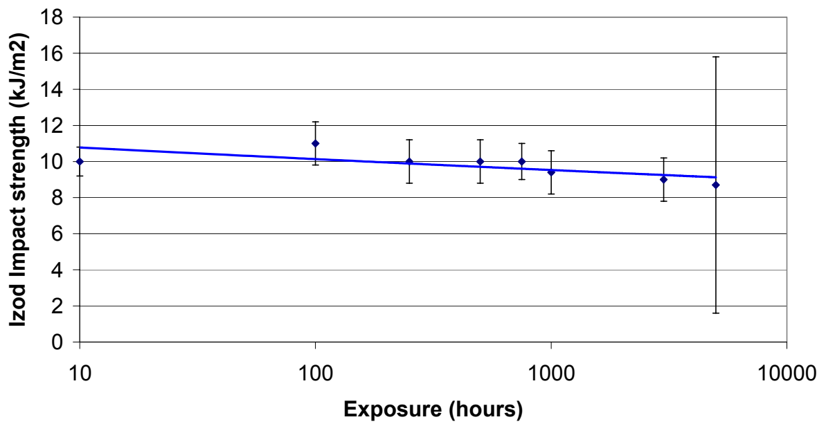
Izod Impact Strength: Wheelie Bin Black
