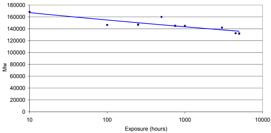
Weight Average Molecular weight: Centriforce Blue
