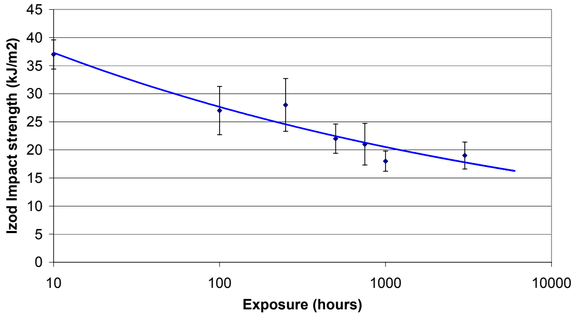
Izod Impact Strength: BPI Rectangular
