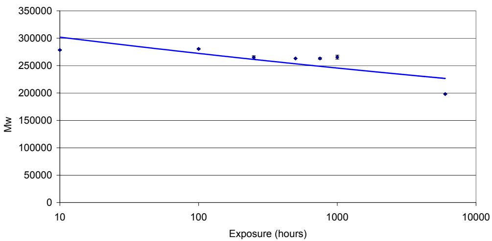
Weight Average Molecular weight: PP Bumper
