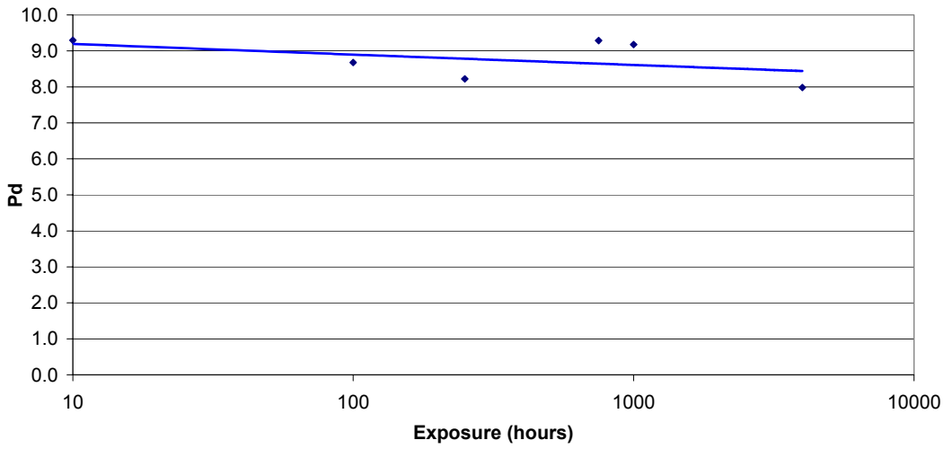
Polydispersity (Mw/Mn): Centriforce Black
