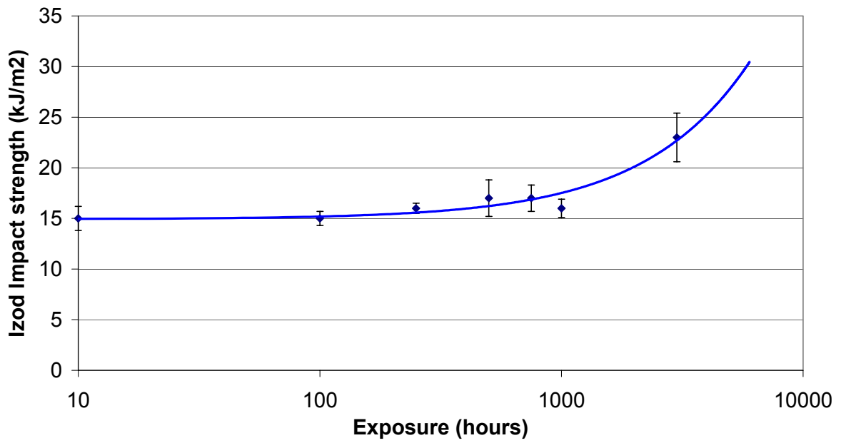
Izod Impact Strength: Centriforce Brown
