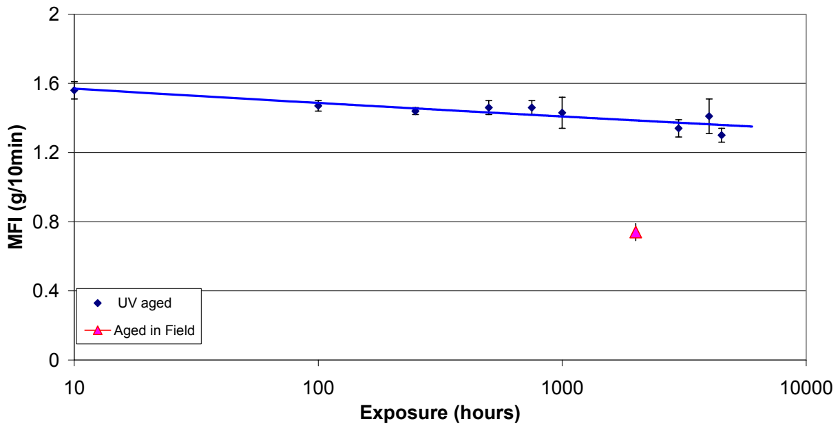
Melt Flow Index: BPI Rectangular
