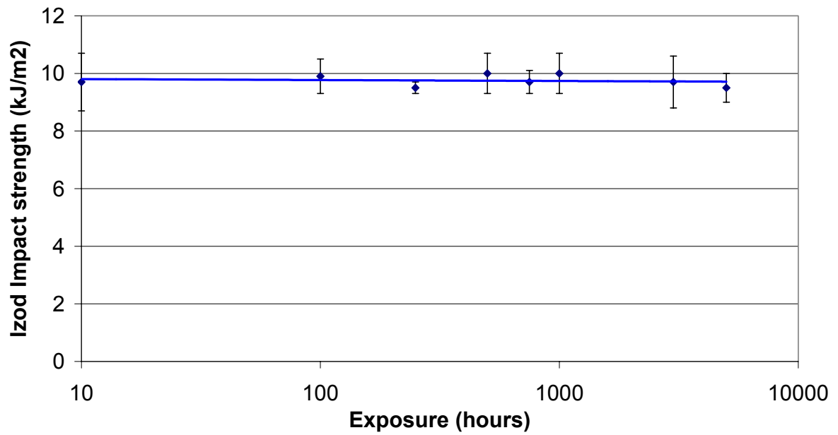
Izod Impact Strength: Wheelie Bin Green
