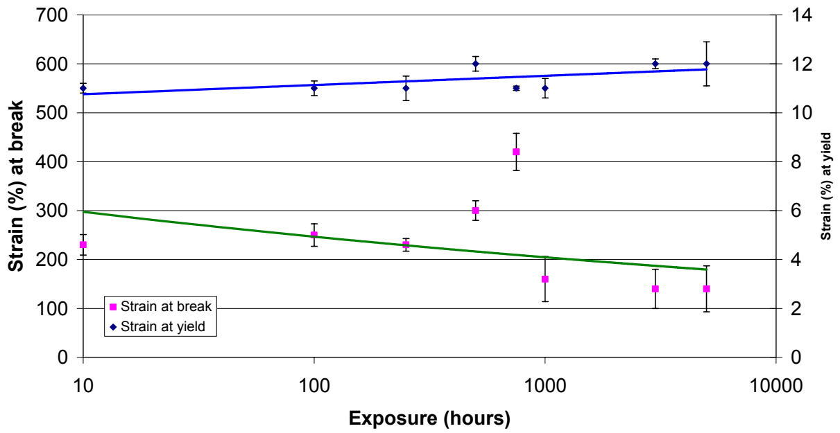
Tensile Strain: Wheelie Bin Black
