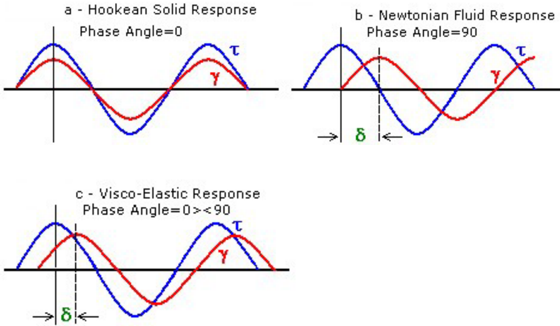
Figure 12 Phase response of fluids under oscillating stress.
