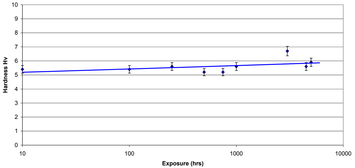
Vickers micro-hardness : Centriforce Brown
