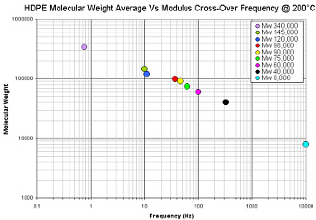
Figure 15: G' and G'' crossover frequency vs molecular weight for HDPE.
