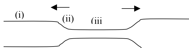
Figure 9: Development of a neck at the onset of cold drawing
