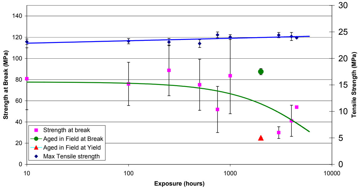
Tensile Strength: Centriforce Black
