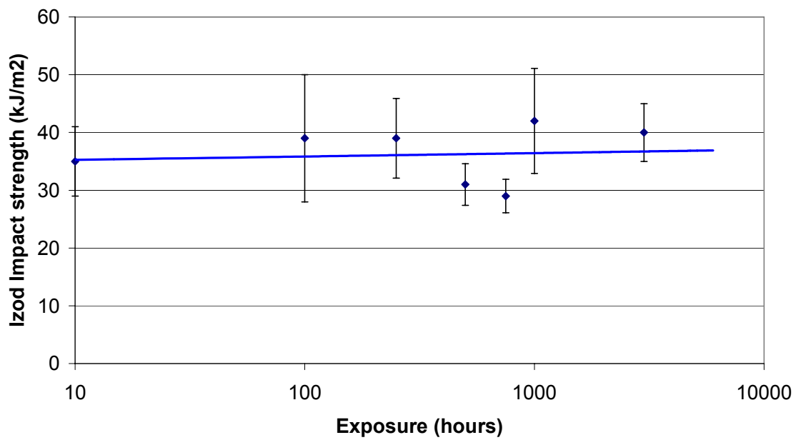
Izod Impact Strength: Centriforce Blue
