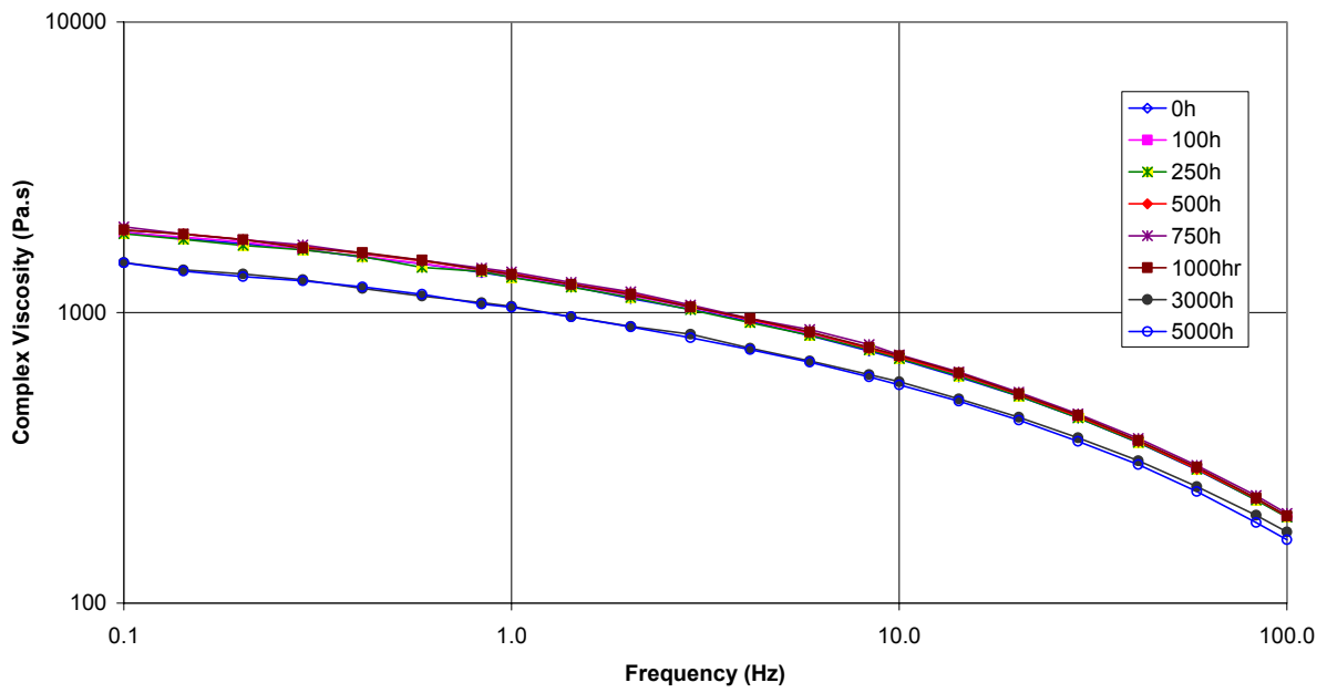
Complex Viscosity Vs Frequency @ 200°C : Wheelie Bin Black
