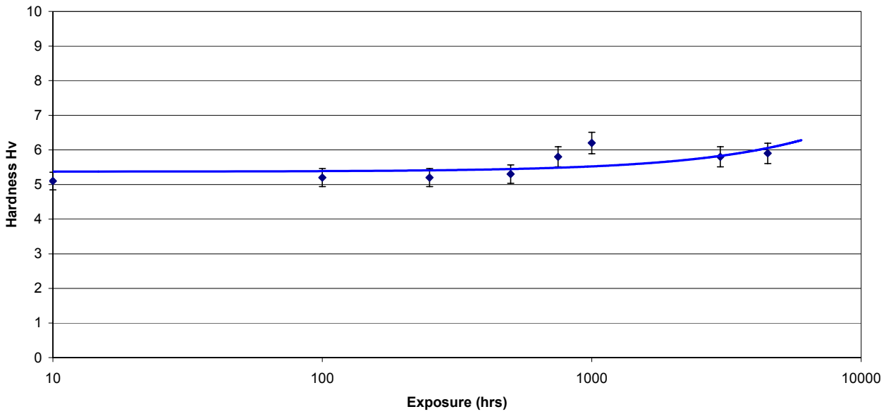
Vickers micro-hardness : Centriforce Blue
