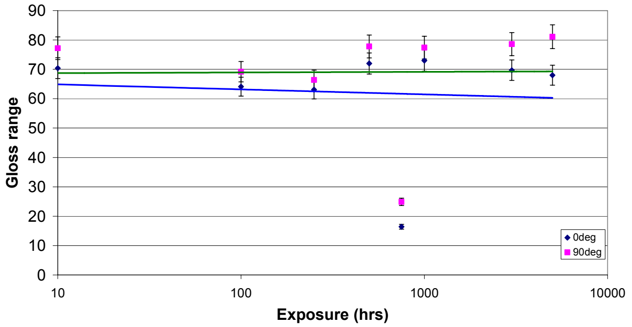
Gloss measurement: Wheelie Bin Green
