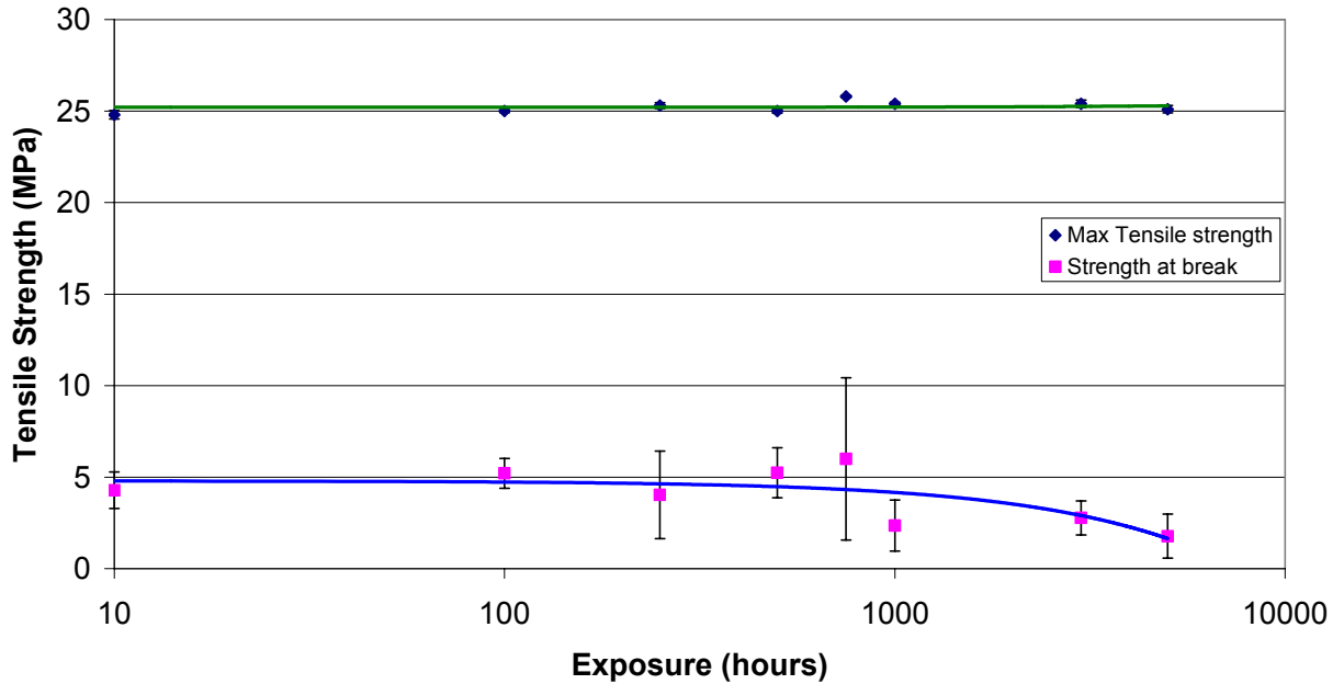
Tensile Strength: Wheelie Bin Black
