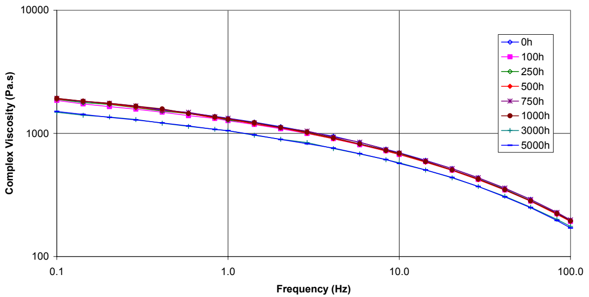
Complex Viscosity Vs Frequency @ 200°C : Wheelie Bin Green
