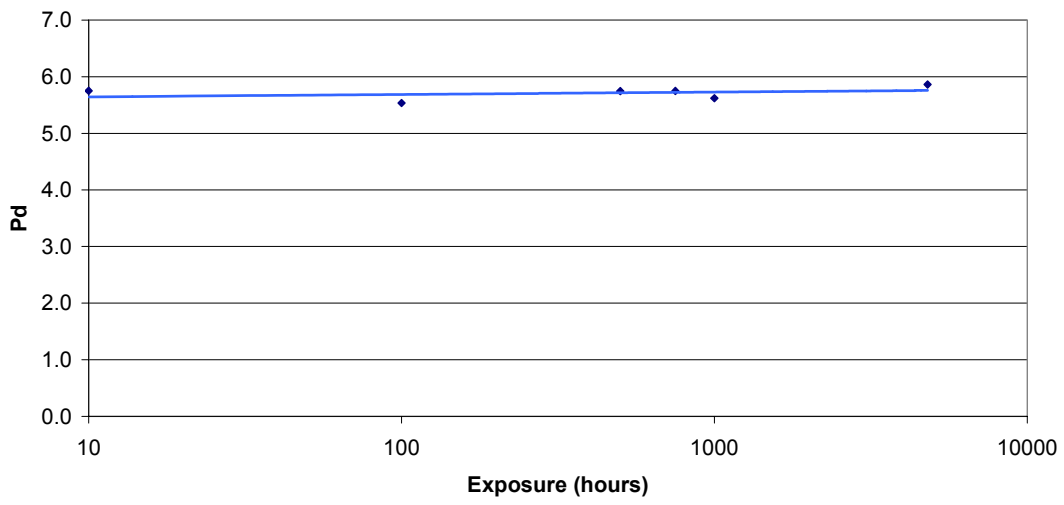
Polydispersity (Mw/Mn): Wheelie Bin Green
