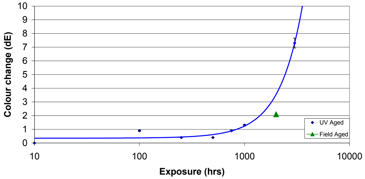
Colour change: BPI Rectangular
