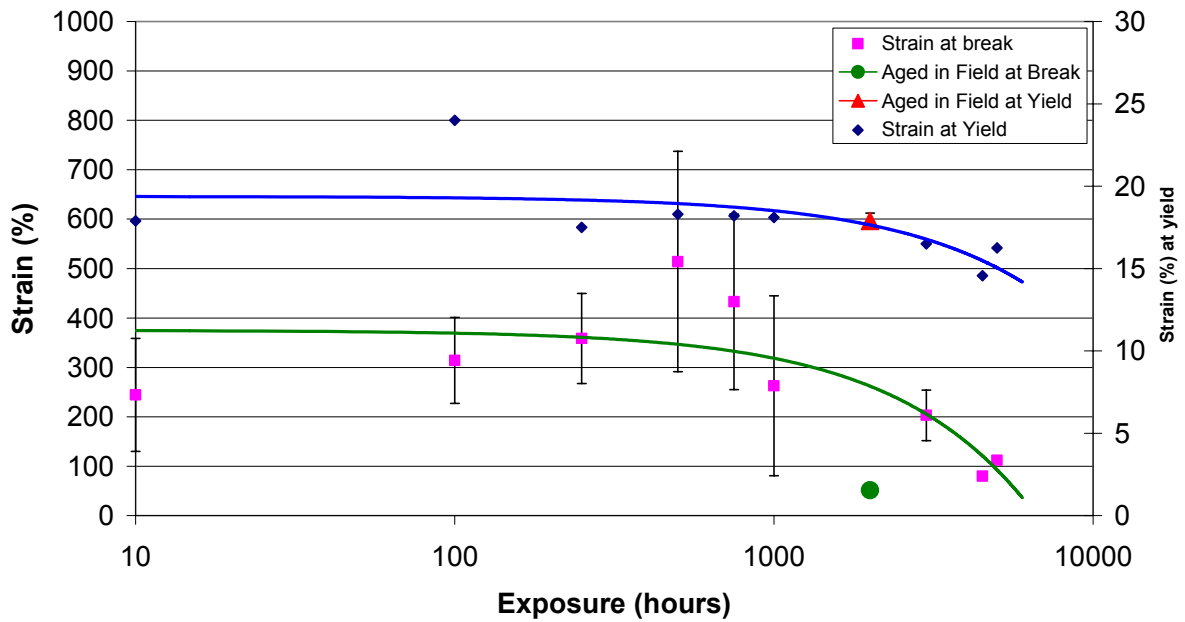
Tensile Strain: Centriforce Blue
