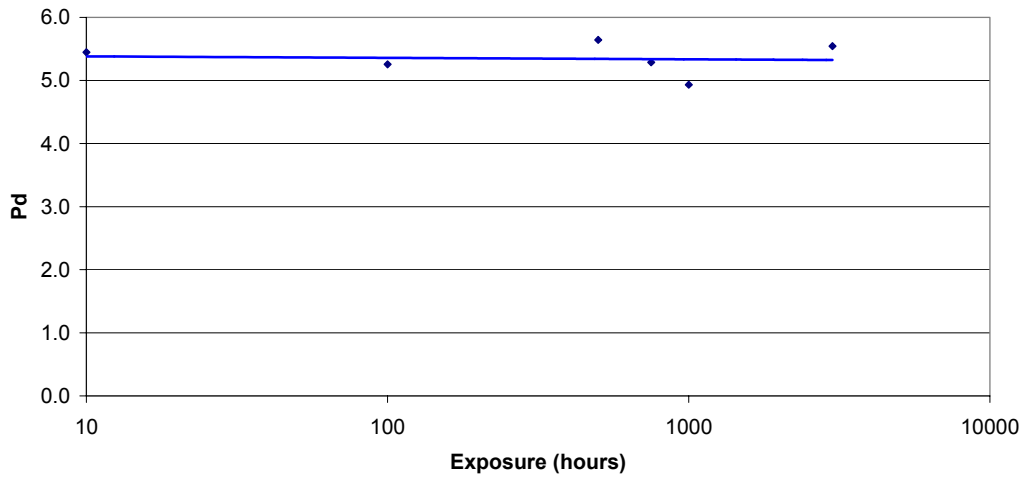
Polydispersity (Mw/Mn): Wheelie Bin Black
