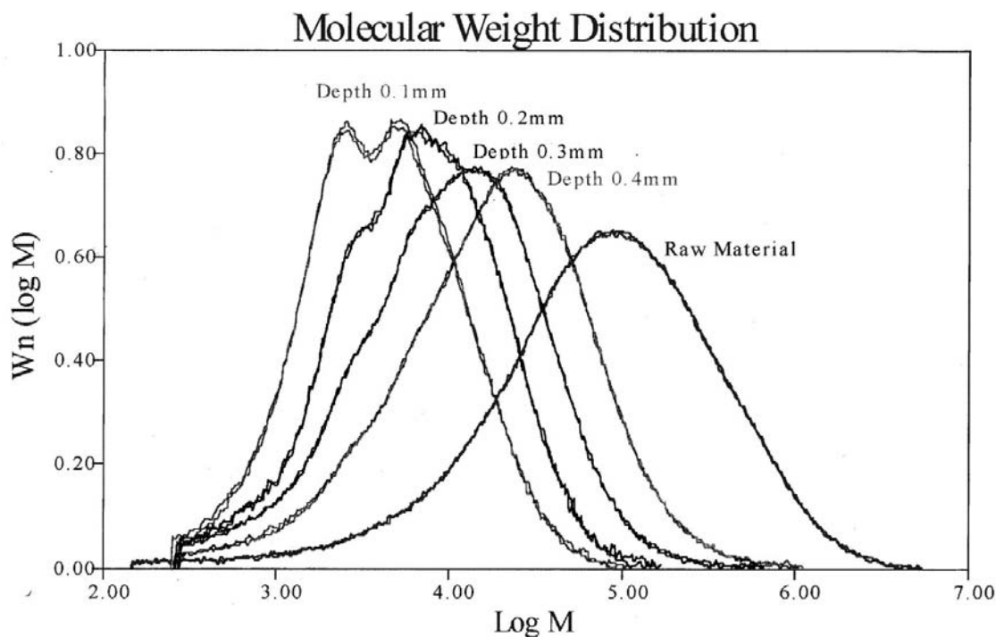
Figure 10 Molecular weight of a PP exposed to UV radiation.
