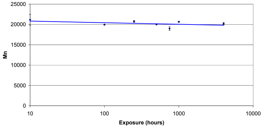
Number Average Molecular Weight: BPI Square
