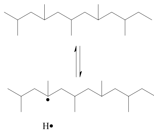
Isotactic Polypropylene
