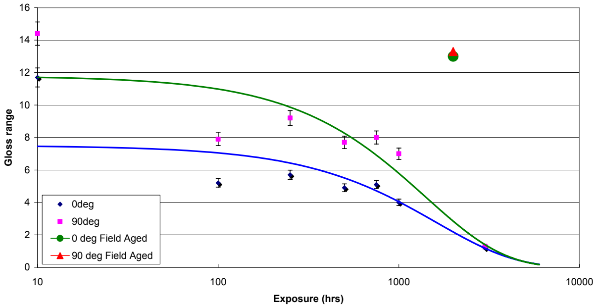
Gloss measurement: BPI Rectangular
