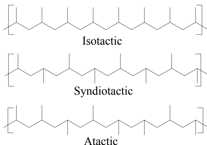
Figure 4: Tacticity of polypropylene
