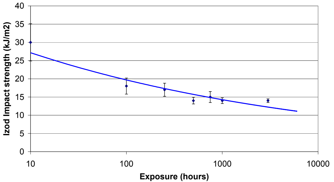
Izod Impact Strength: BPI Square
