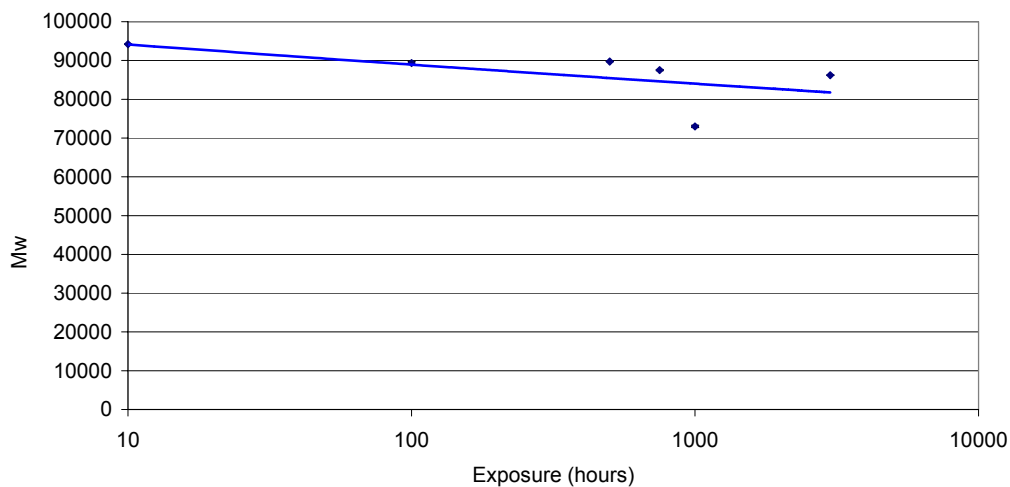
Weight Average Molecular weight: Wheelie Bin Black
