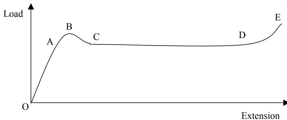
Figure 8: Tensile test behaviour incorporating cold drawing
