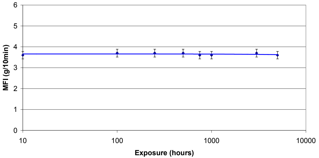
Melt Flow Index: Wheelie Bin Green
