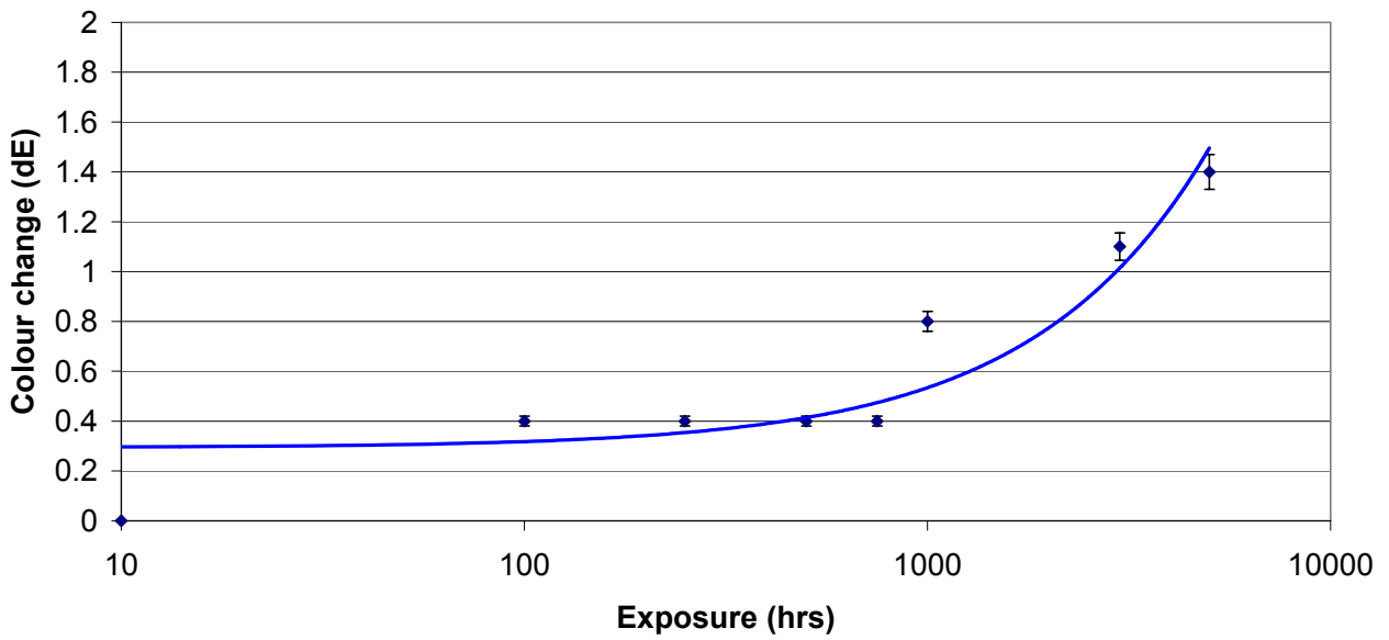
Colour change: Wheelie Bin Green
