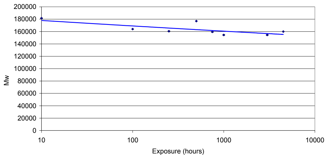
Weight Average Molecular weight: Centriforce Brown
