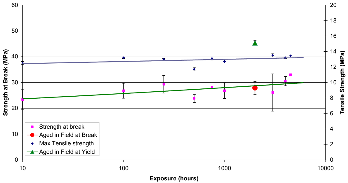
Tensile Strength: BPI Square
