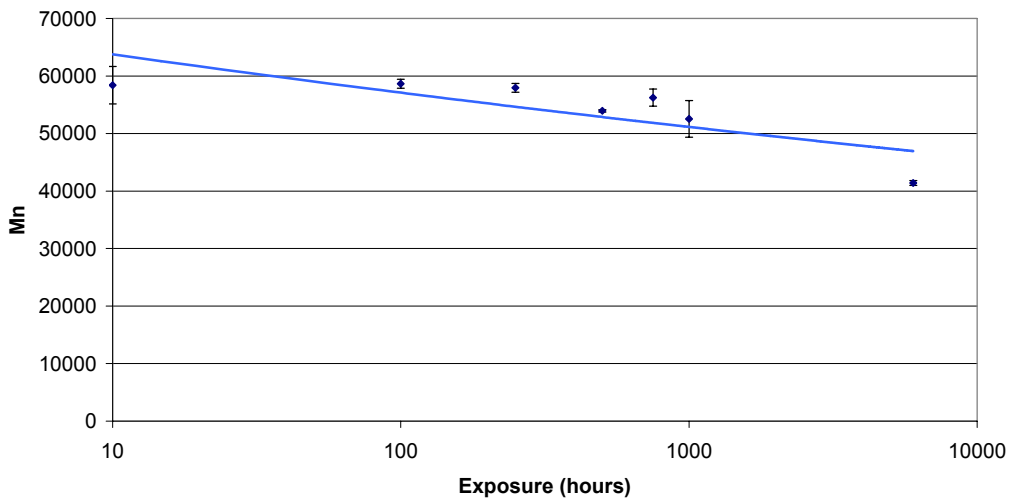
Number Average Molecular Weight: PP Bumper
