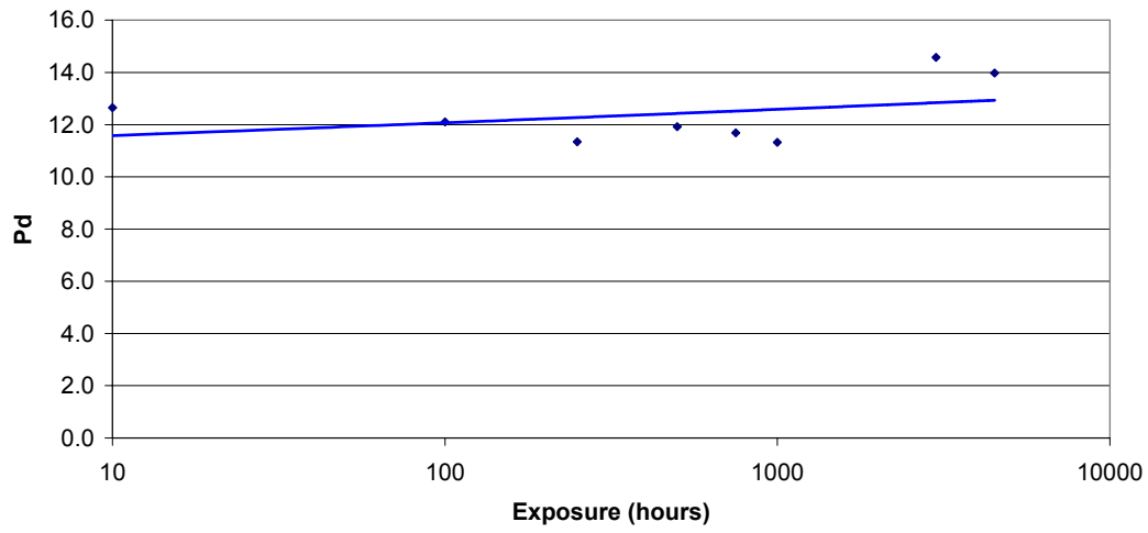
Polydispersity (Mw/Mn): Centriforce Brown
