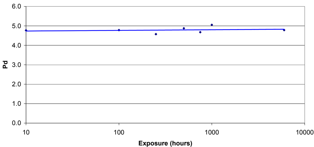
Polydispersity (Mw/Mn): PP Bumper
