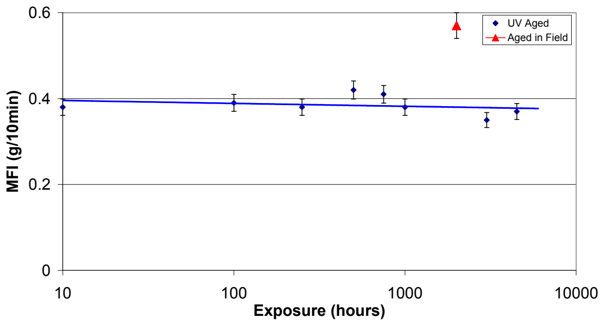
Melt Flow Index: Centriforce Brown
