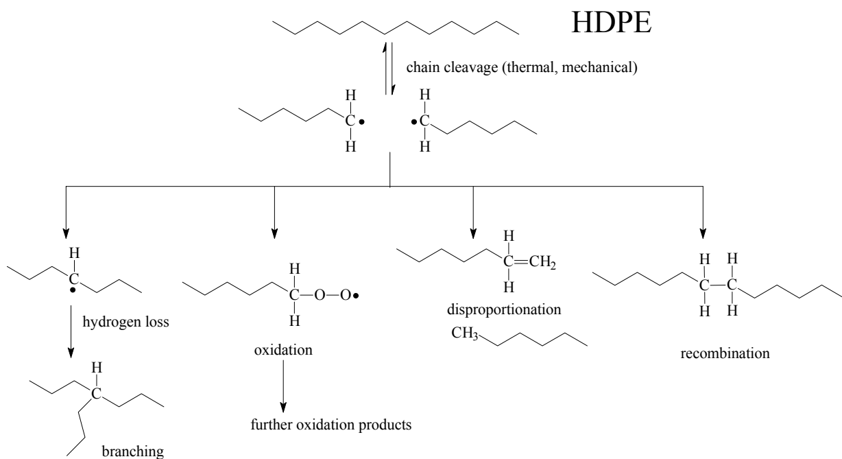
Figure 1: Reactions after thermal processing of polyethylene
