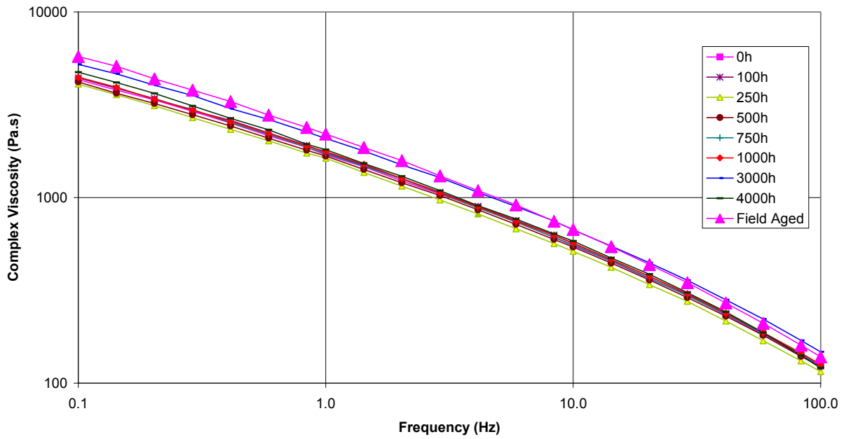
Complex Viscosity Vs Frequency @ 200°C : BPI Square
