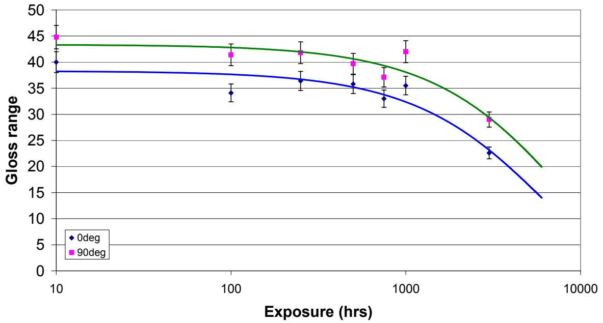
Gloss measurement: Centriforce Brown
