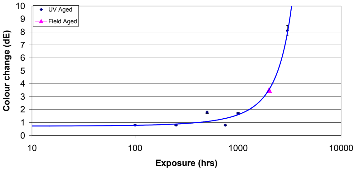
Colour change: BPI Square
