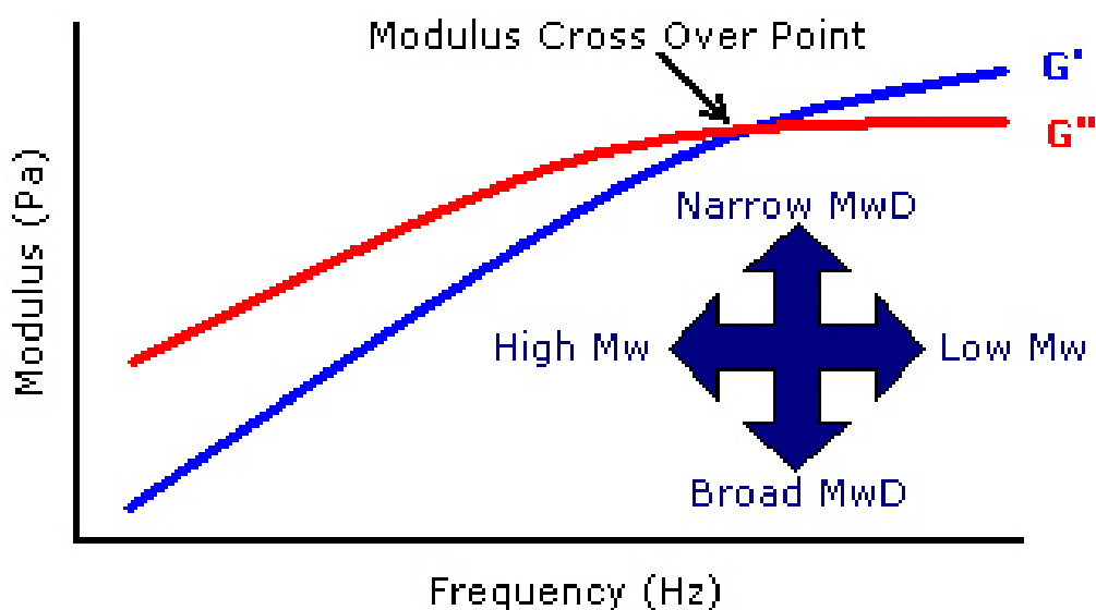
Figure 14 Change in position of the G'/G'' crossover point with molecular weight.
