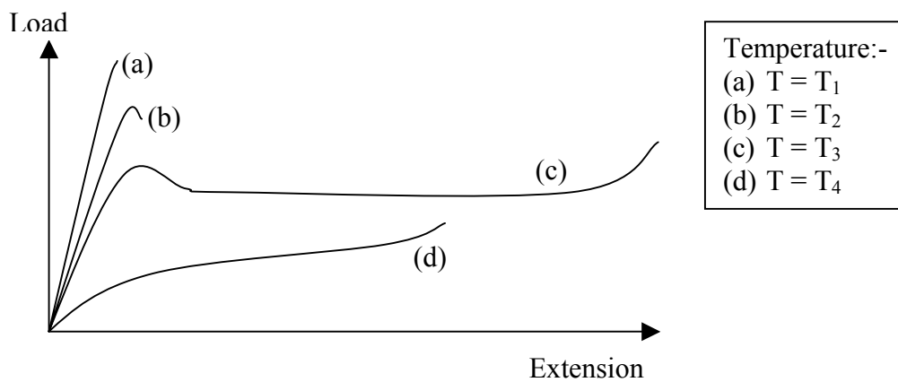
Figure 7: Typical Test results for solid polymers
