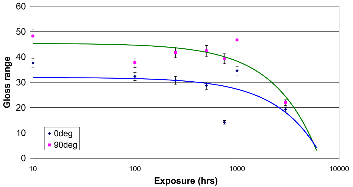
Gloss measurement: Centriforce Blue
