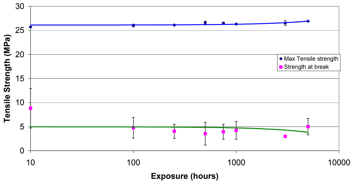
Tensile Strength: Wheelie Bin Green
