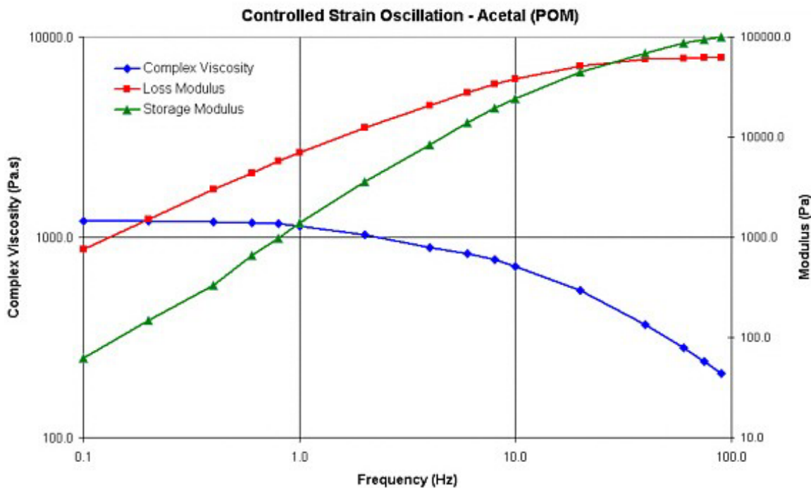
Figure 13 Typical results generated for an acetal.
