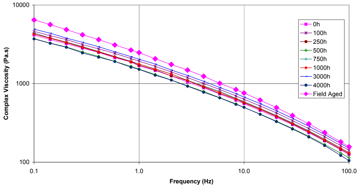
Complex Viscosity Vs Frequency @ 200°C : BPI Rectangular
