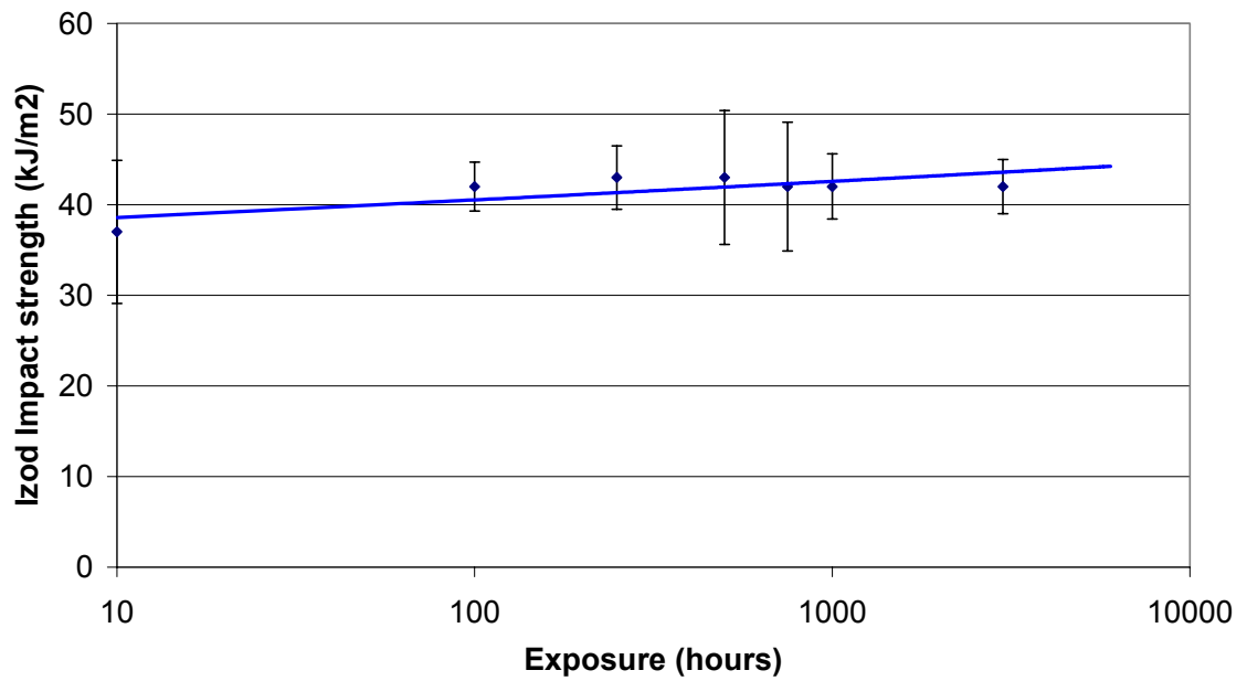
Izod Impact Strength: PP Bumper
